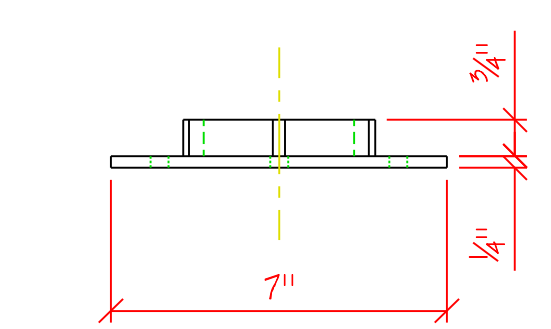
BASE PLATE DETAIL SCALE: 3/4"=1'-0"
