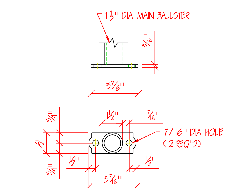
DETAIL III SCALE: 3/4"=1'-0"
