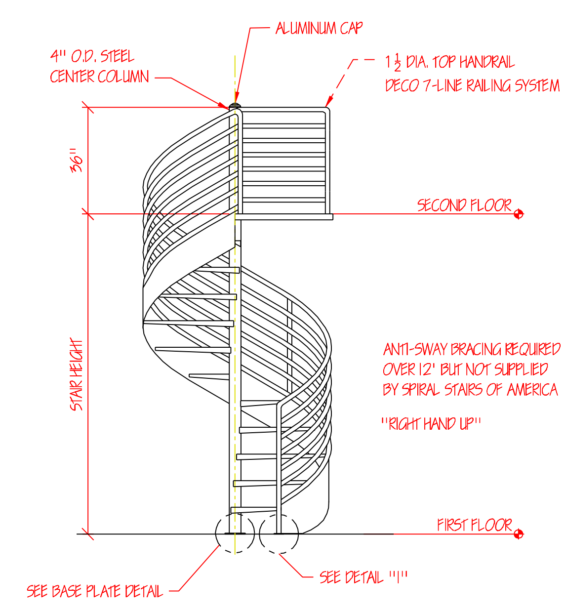
SIDE ELEVATION SCALE: 3/8"=1'-0"
