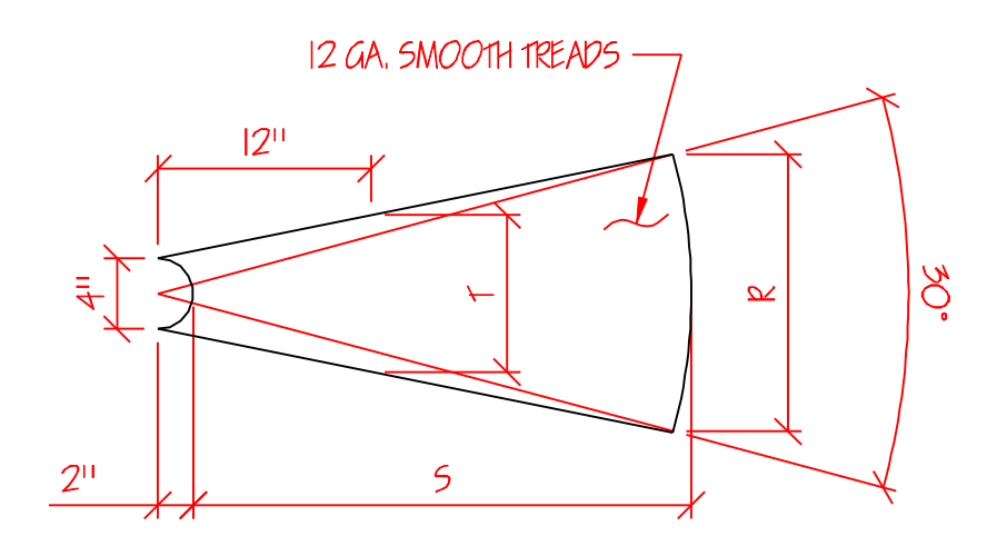
RADIUS TREAD DETAIL SCALE: 1"=1'-0"
