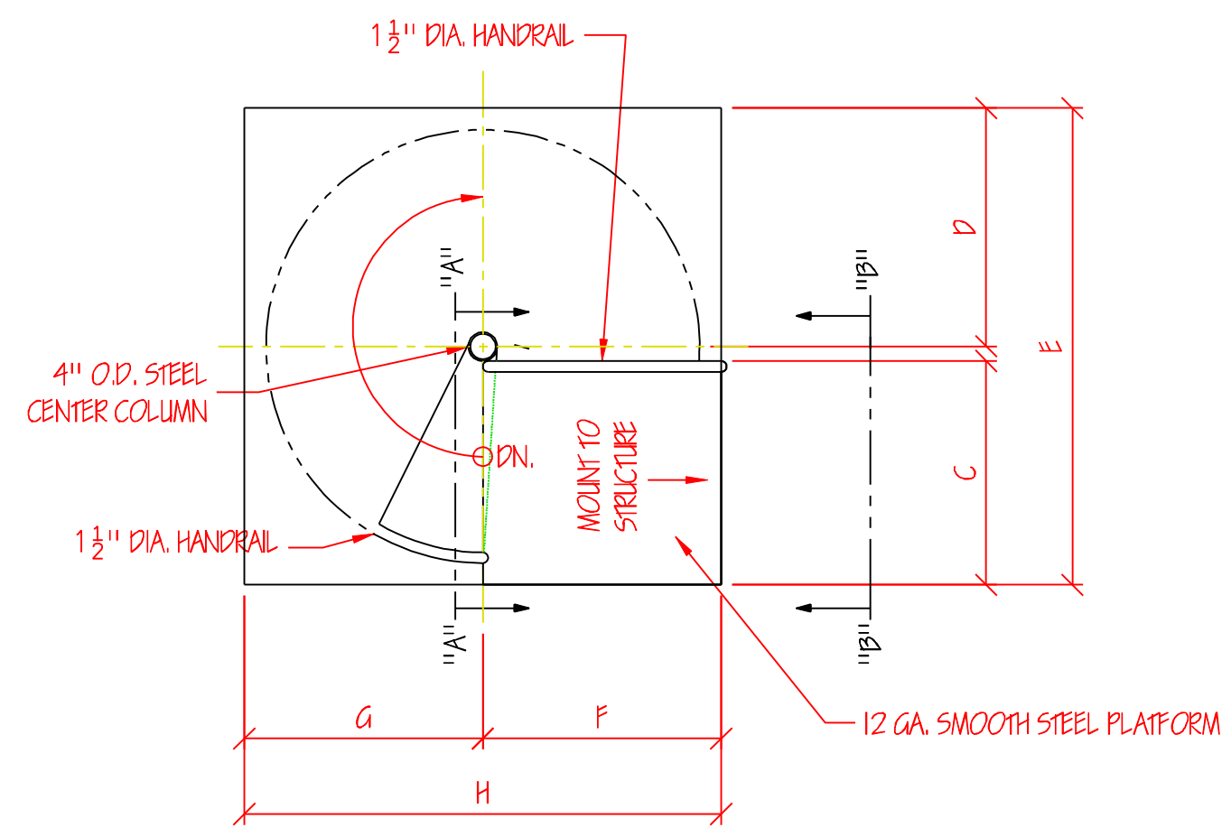
PLAN VIEW AT TOP STAIR SCALE: 1/2"=1'-0"
