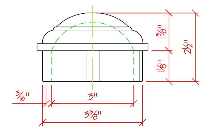
ALUMINUM CAP DETAIL SCALE: 6"=1'-0"
