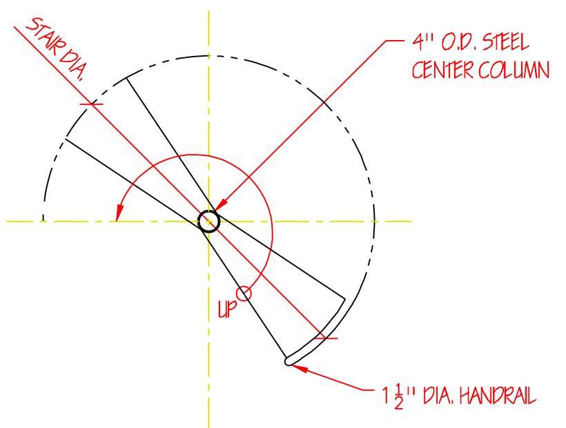
PLAN VIEW AT BOTTOM SCALE: 1/2"=1'-0"
