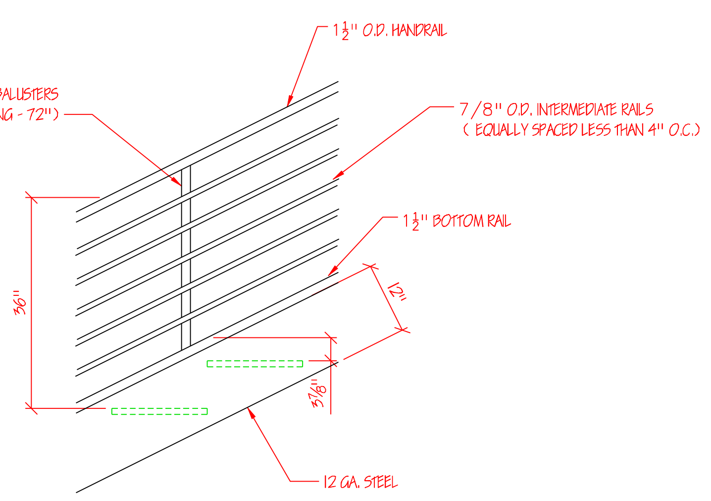
BALUSTER DETAIL SCALE: 3/4"=1'-0"
