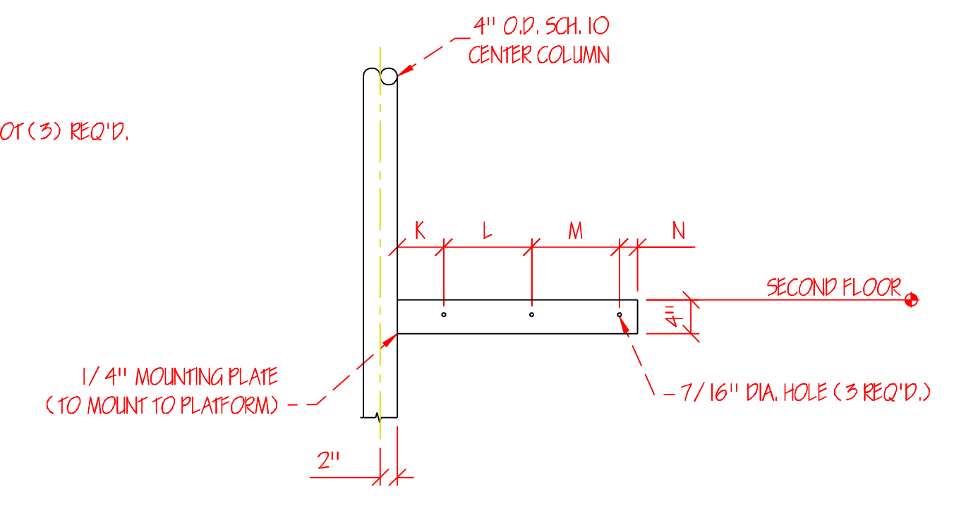
MOUNTING PLATE DETAIL SCALE: 3/4"=1'-0"
