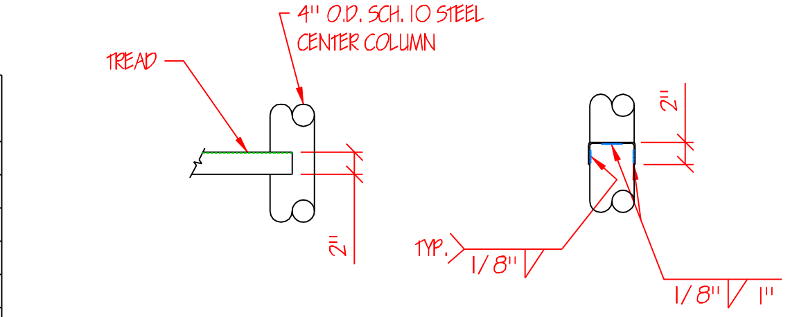
TREAD WELD DETAIL SCALE: 1"=1'-0"
