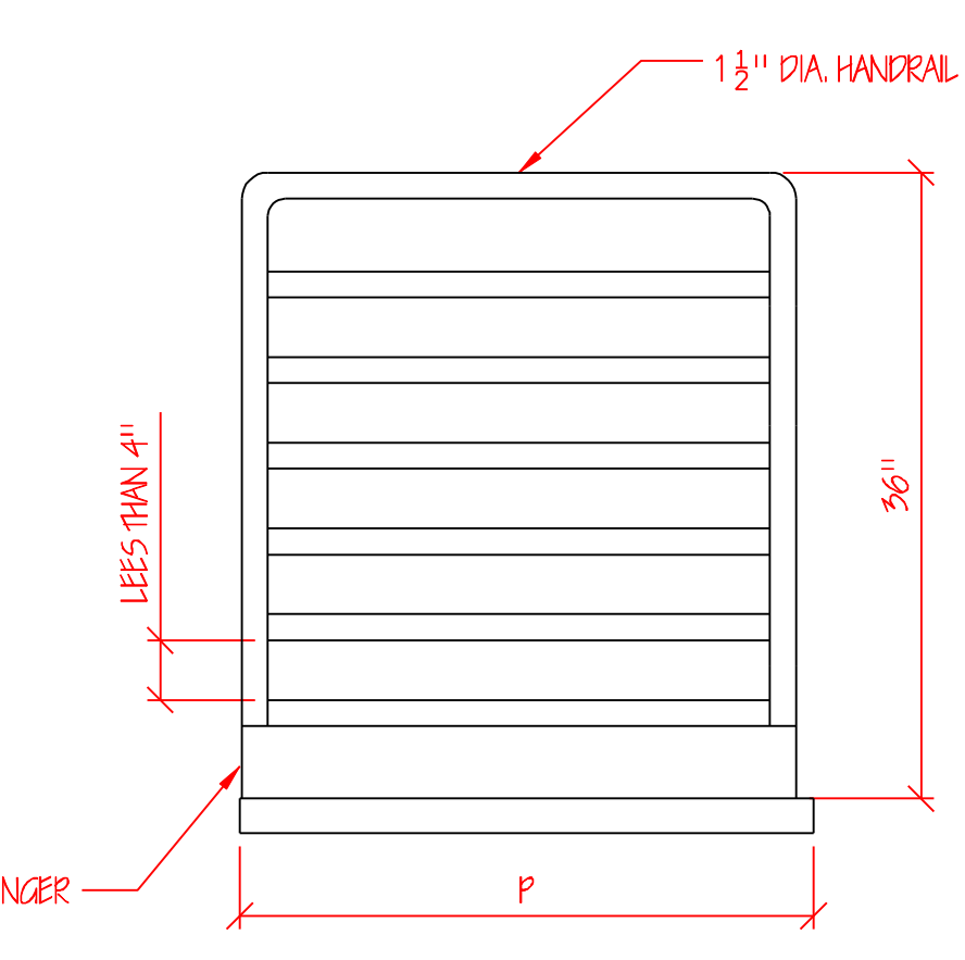
PLATFORM DETAIL SCALE: 1"=1'-0"
