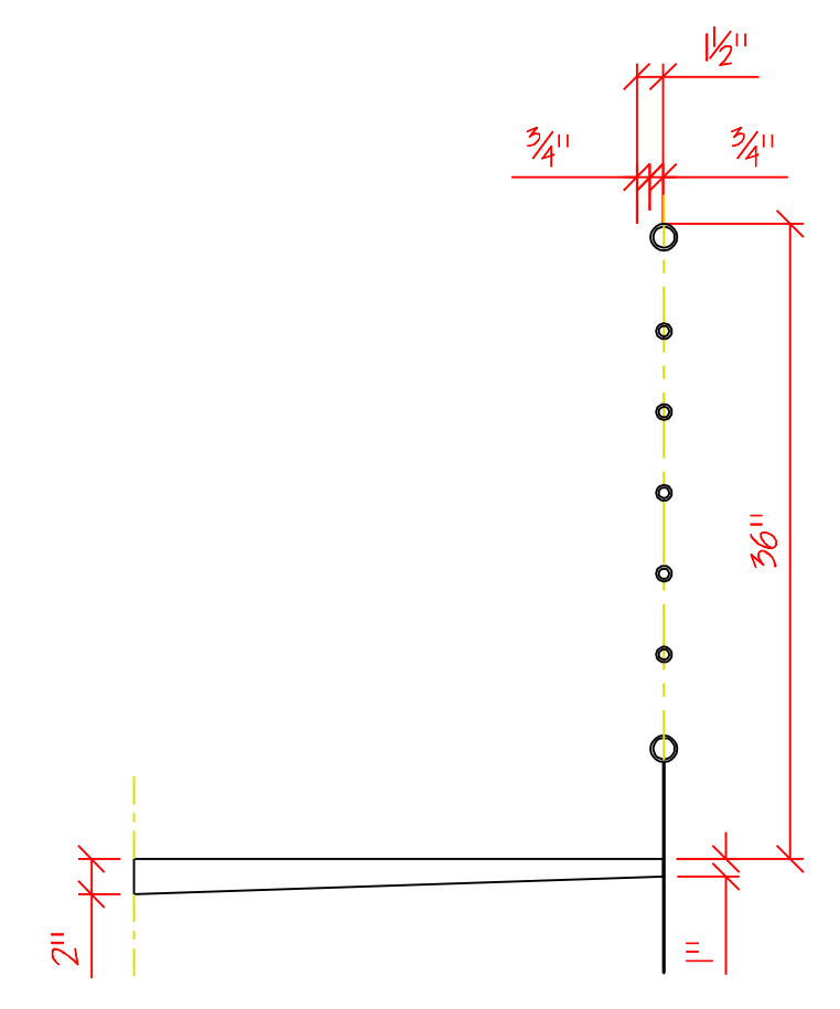
TREAD WELD DETAIL SCALE: 1"=1'-0"
